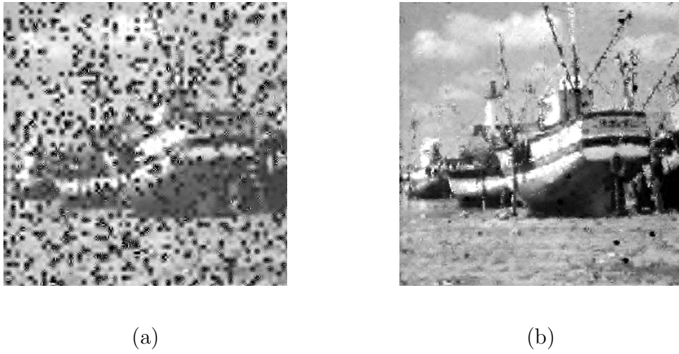
Figure 3.7. Comparison between direct CS and CopCS, a\% = 10\% . (a) recovered image via direct CS, (b) recovered image via CopCS with (3, 4).
