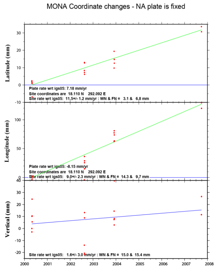
Figure 3.25 Time series for site MONA. Red dots are the UTC daily position solutions. The blue lines are the predicted plate rates in ITRF05 held fixed (horizontal). The green lines are the least square fit site rates in IGS05 (a) with respect to the Caribbean plate rate-CA and (b) with respect to the North-American plate rate-NA. WN = white noise; FN = flicker noise estimates.
