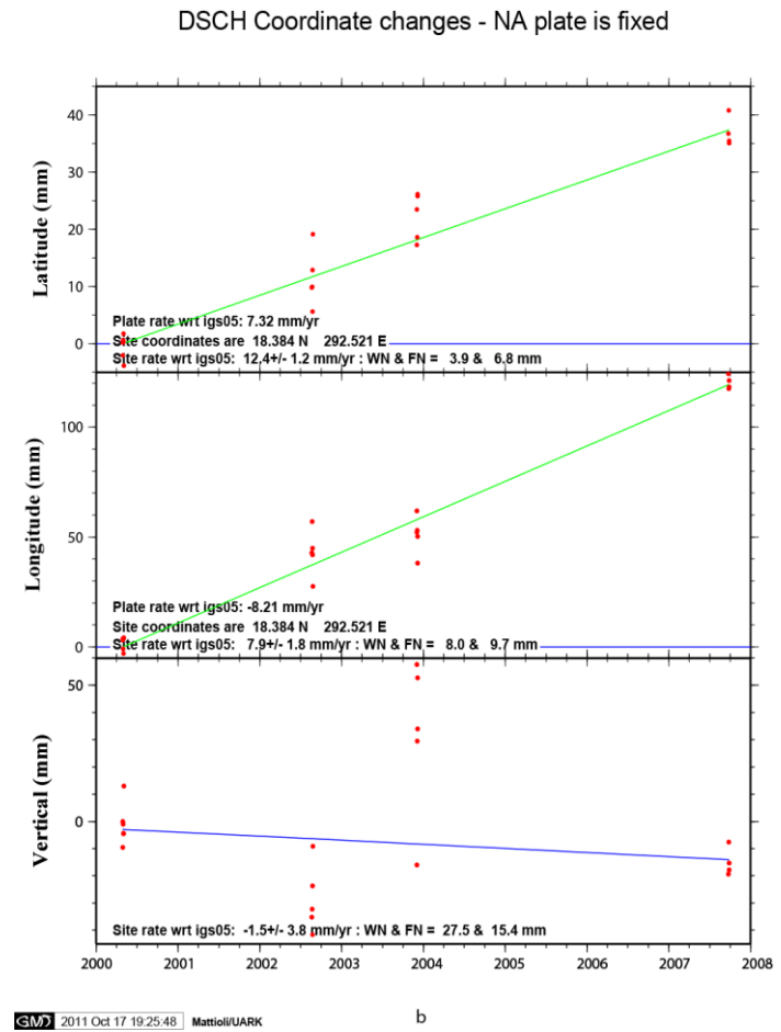
Figure 3.30 Time series for site DSCH. Red dots are the UTC daily position solutions. The blue lines are the predicted plate rates in ITRF05 held fixed (horizontal). The green lines are the least square fit site rates in IGS05 (a) with respect to the Caribbean plate rate-CA and (b) with respect to the North-American plate rate-NA. WN = white noise; FN = flicker noise estimates.
