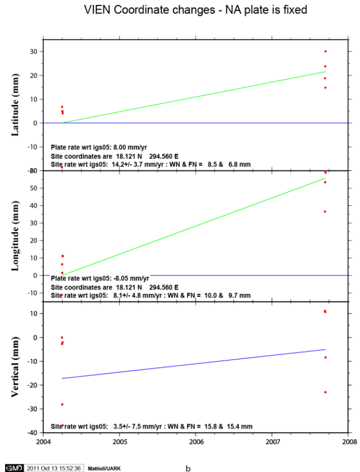
Figure 3.27 Time series for site VIEN. Red dots are the UTC daily position solutions. The blue lines are the predicted plate rates in ITRF05 held fixed (horizontal). The green lines are the least square fit site rates in IGS05 (a) with respect to the Caribbean plate rate-CA and (b) with respect to the North-American plate rate-NA. WN = white noise; FN = flicker noise estimates.
