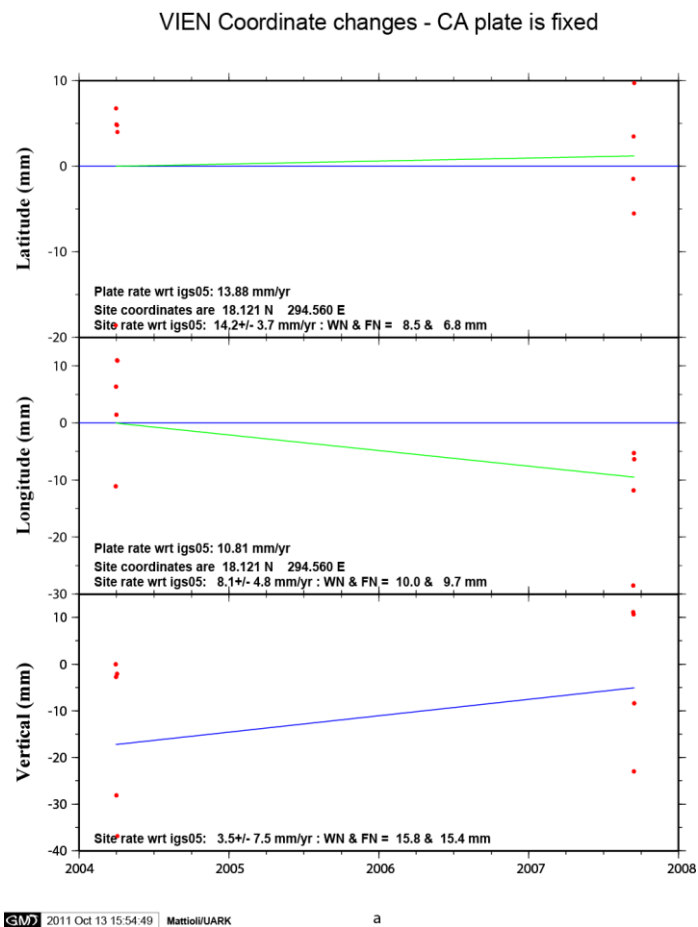
Figure 3.27 Time series for site VIEN. Red dots are the UTC daily position solutions. The blue lines are the predicted plate rates in ITRF05 held fixed (horizontal). The green lines are the least square fit site rates in IGS05 (a) with respect to the Caribbean plate rate-CA and (b) with respect to the North-American plate rate-NA. WN = white noise; FN = flicker noise estimates.
