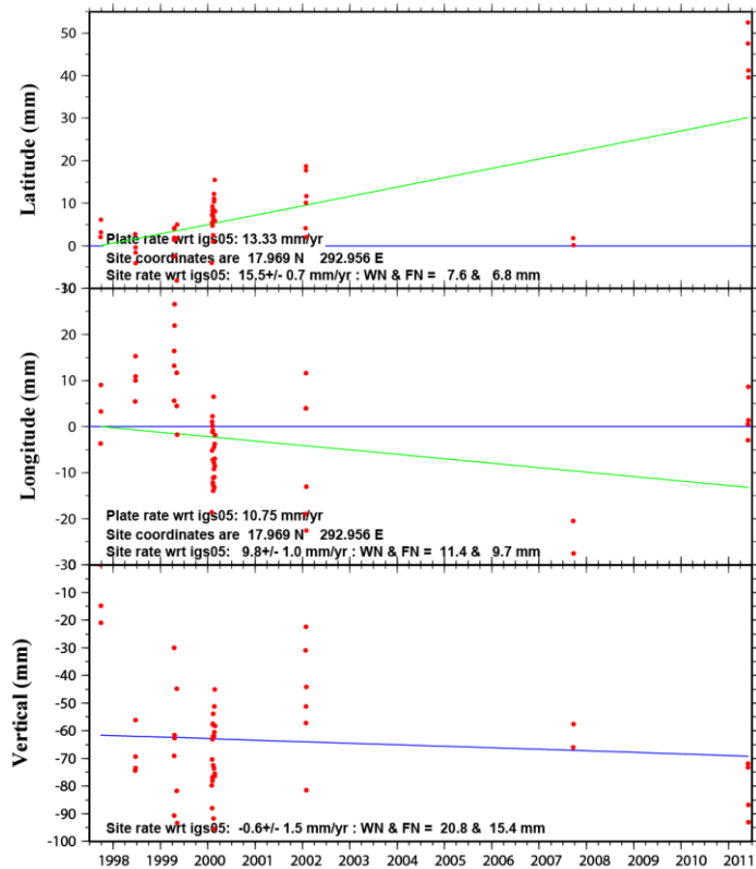
PARG Coordinate changes - CA plate is fixed
