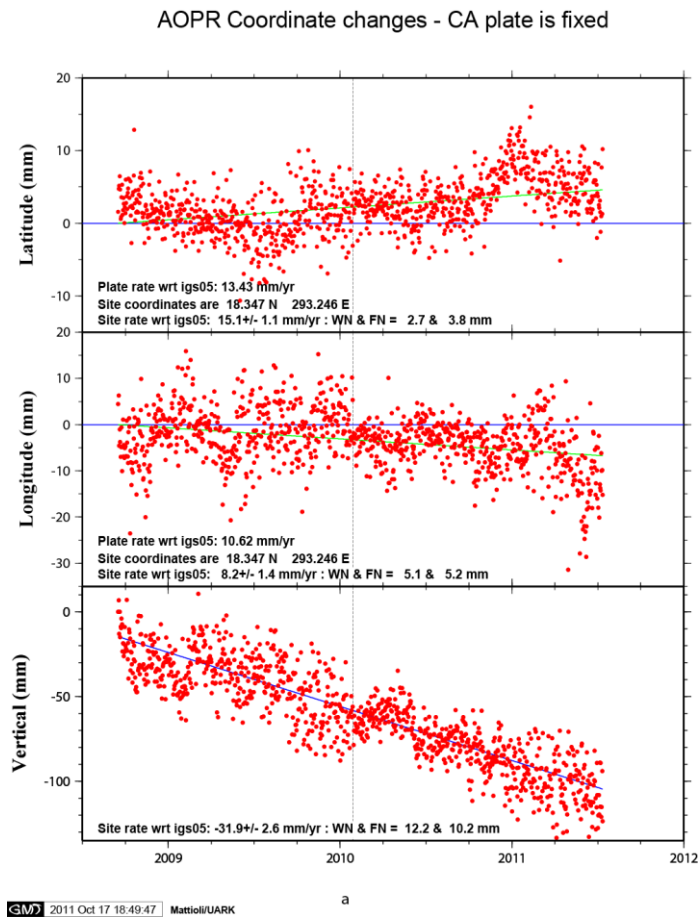
Figure 3.2 Time series for site AOPR. Red dots are the UTC daily position solutions. The blue lines are the predicted plate rates in ITRF05 held fixed (horizontal). The green lines are the least square fit site rates in IGS05 (a) with respect to the Caribbean plate rate-CA and (b) with respect to the North-American plate rate-NA. WN = white noise; FN = flicker noise estimates.
