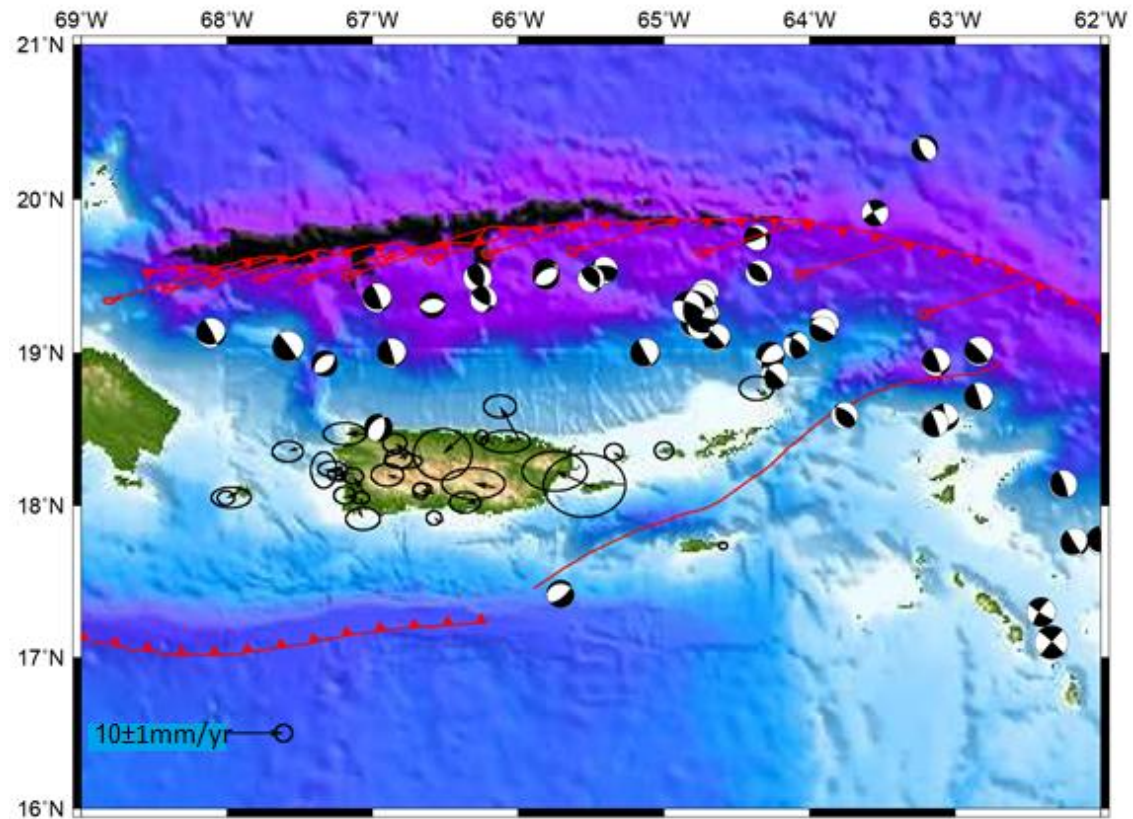
Figure 3.35 Velocity Map of Puerto Rico-Virgin Islands with respect to stable Caribbean Plate
