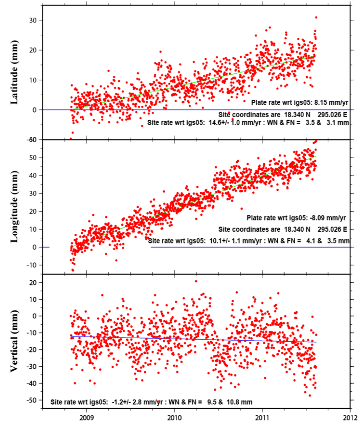
STVI Coordinate changes - NA plate is fixed
