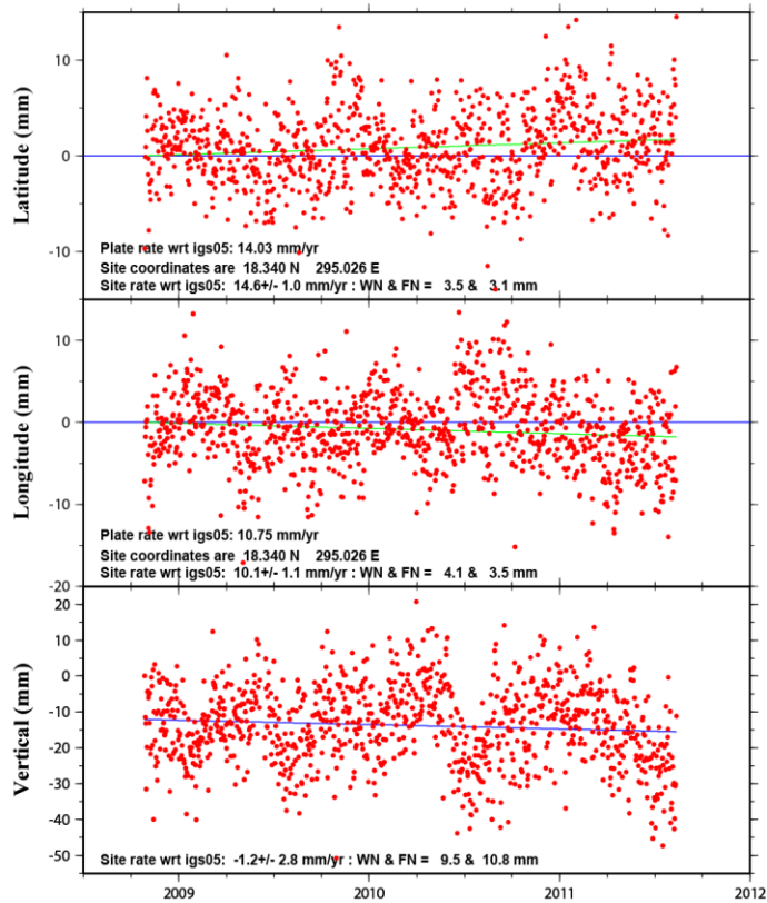
STVI Coordinate changes - CA plate is fixed
