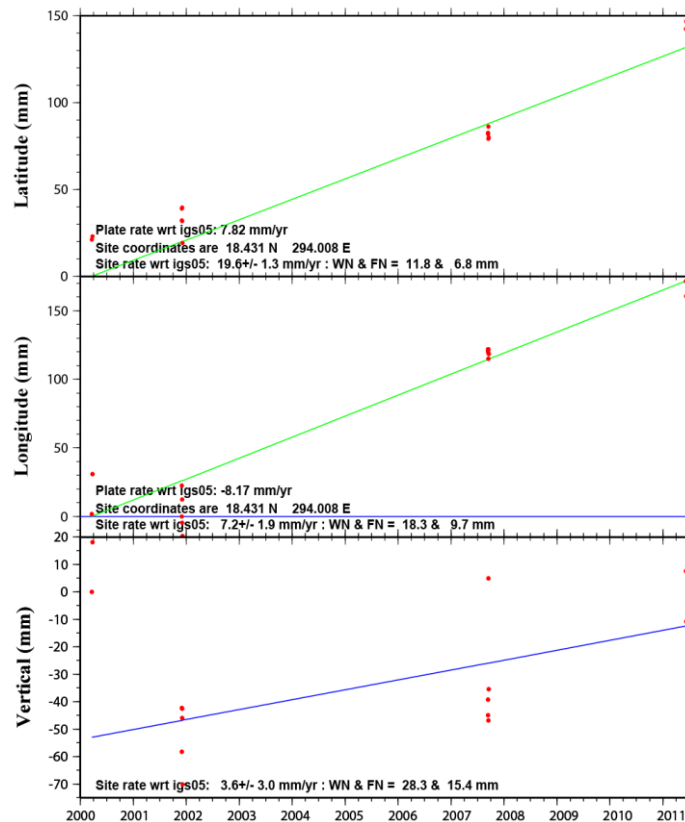
ZSUB Coordinate changes - NA plate is fixed
