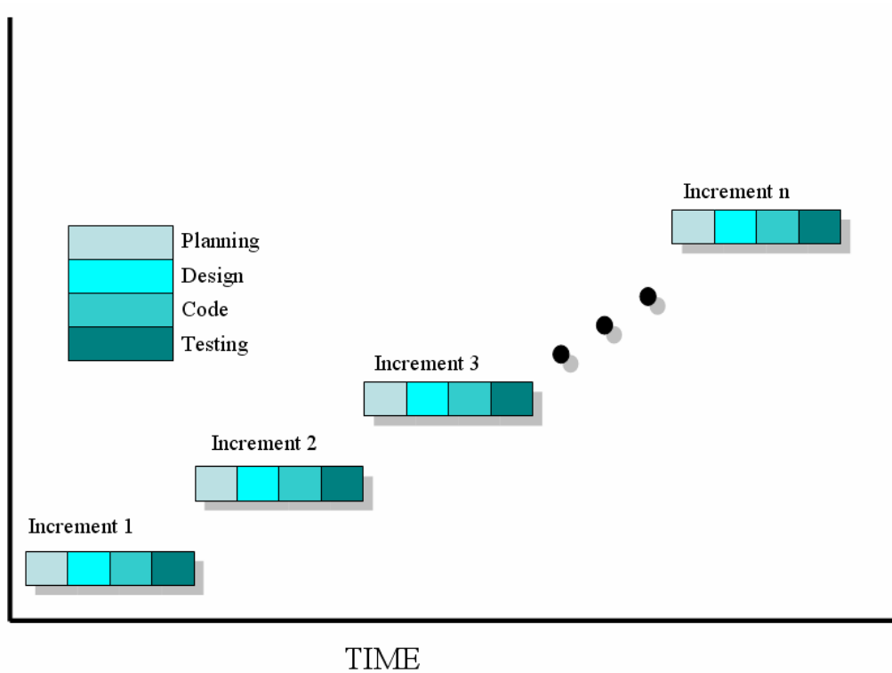
Figure 2.5 XP [LOF05]
